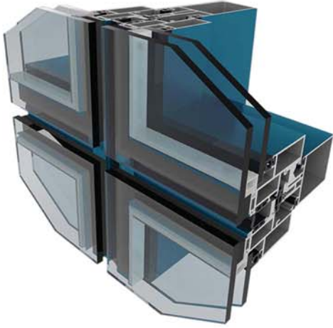
SC-50 SİLİKON CEPHE SİSTEMİ (silicone facade system)
