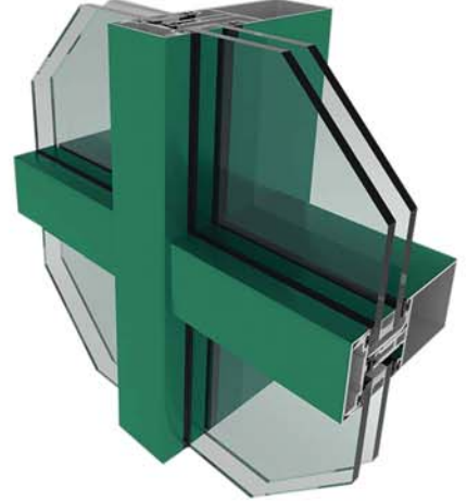
KC-50 KAPAKLI CEPHE SİSTEMİ (frame facade system)
