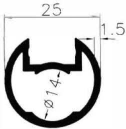
3626 0.363 Kg/m
