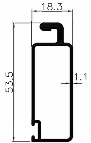
7455 ●.486 Kg/m
