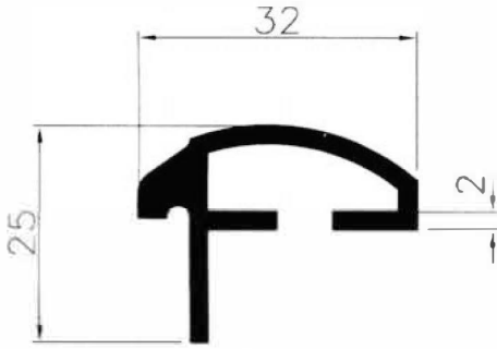
4396 0.460 Kg/m
