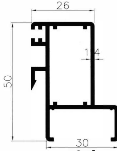
1902 0.693 Kg/m
