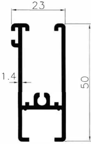
1899 0.588 Kg/m
